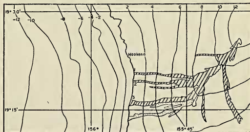
FIG. 1. Land areas covered by the Mauna Loa lava flows of 1919 and 1950. Heights above and below sea level given in thousands of feet. Diagonally hatched areas: 1950 flows; those that entered the sea are numbered in the sequence with which they reached sea level. Stippled area: 1919 flow. Redrafted in part from Macdonald and Finch.
